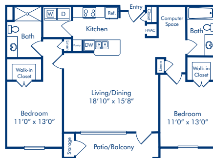
Model B2 2 Bedroom/2 Bath 1136 Sq. Ft.
